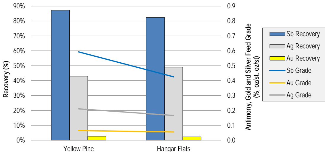
Figure 1.3: Antimony Concentrate Recoveries
